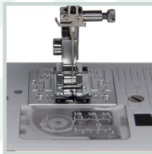
4-piece feed dog
