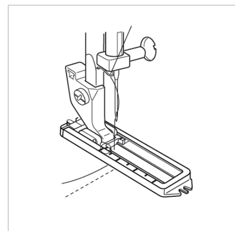
Buttonhole foot
